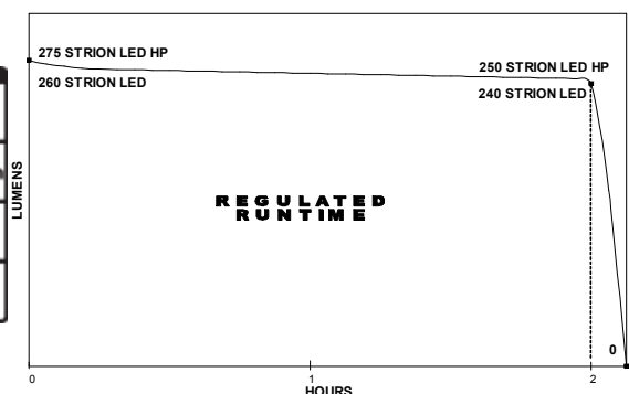
PERFORMANCE CURVE
